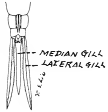
Fig. 145. Dorsal aspect of abdominal segments of a damselfly naiad.
